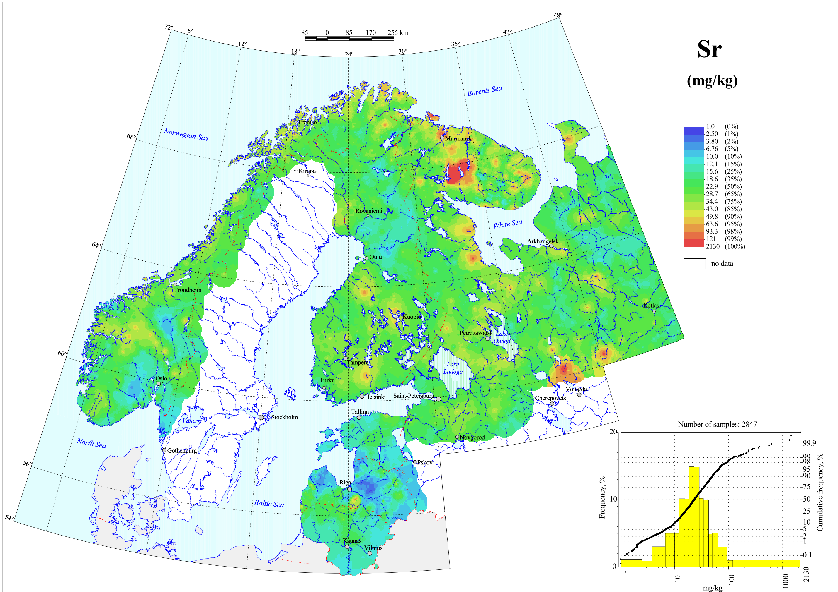
Strontium in Organic Soil Layer, Total Content
